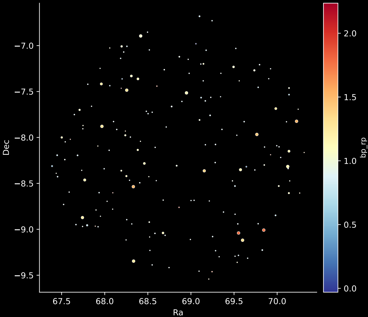
APOGEE DR17 Field: [049-44_MGA] Stars: 172
