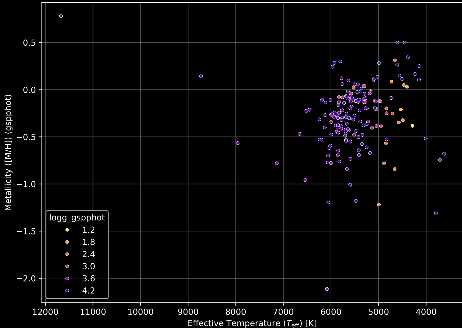
APOGEE DR17 Field: [049-44_MGA] Stellar Population Parameters (n= 172)
