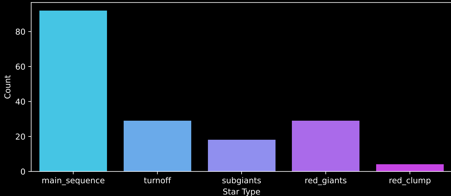
APOGEE DR17 Field: [049-44_MGA] Count plot of Star Type
