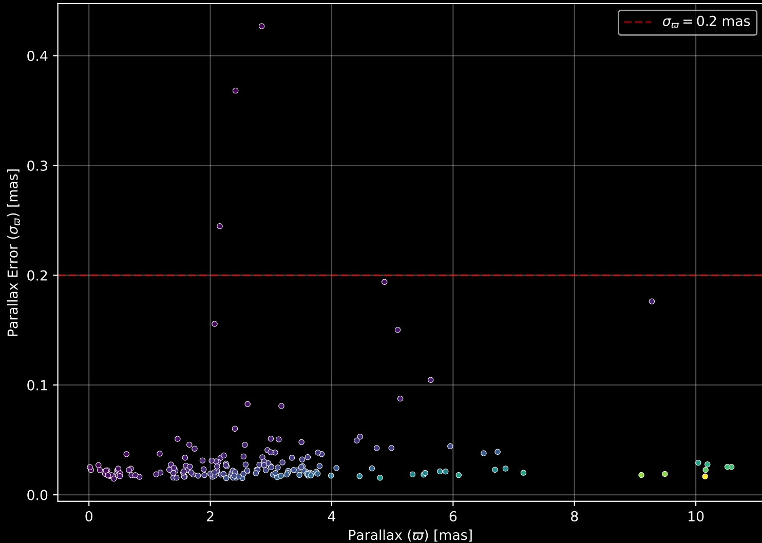
APOGEE DR17 Field: [049-44_MGA] Parallax Quality (n= 172)
