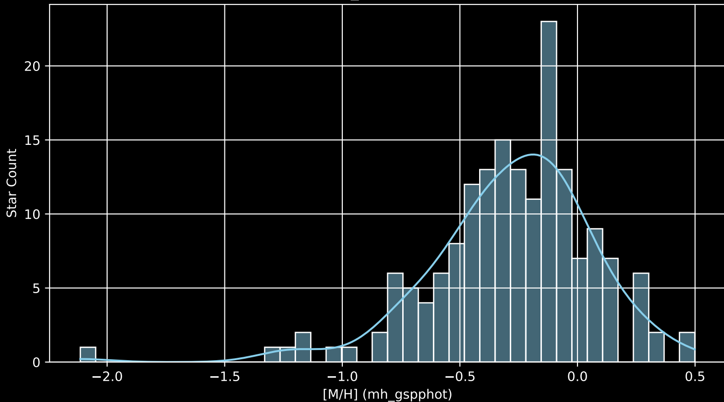
APOGEE DR17 Field: [049-44_MGA [M/H] (mh_gspphot) (n= 171)
