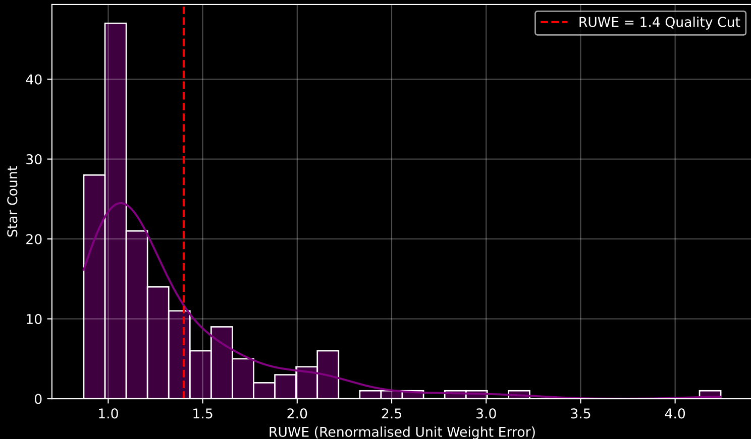
GAPOGEE DR17 Field [049-44_MGA] RUWE Distribution (n= 163)
