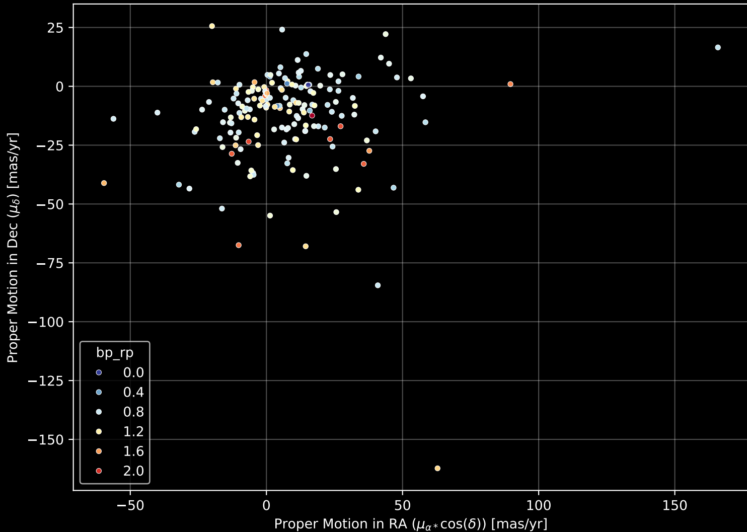
APOGEE DR17 Field: [049-44_MGA] Proper Motion Diagram (n= 172)
